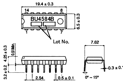
BU4584B(DIP14)(UNIT:[mm])
