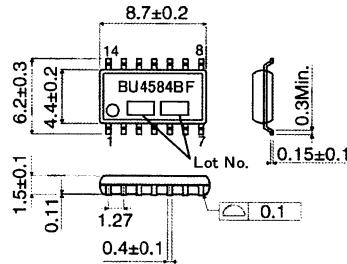
BU4584BF(SOP14)(UNIT:[mm])
